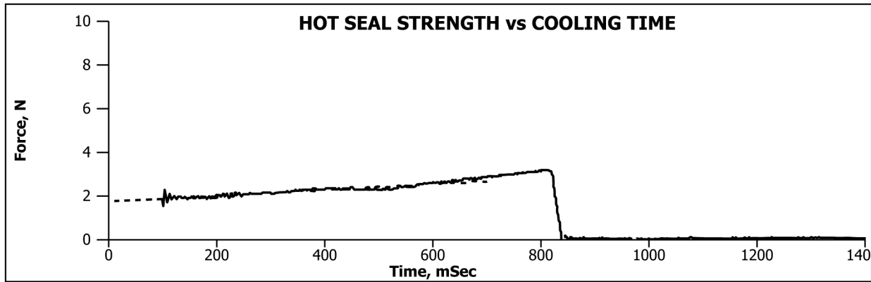
FIG. 2 Cooling Curve
