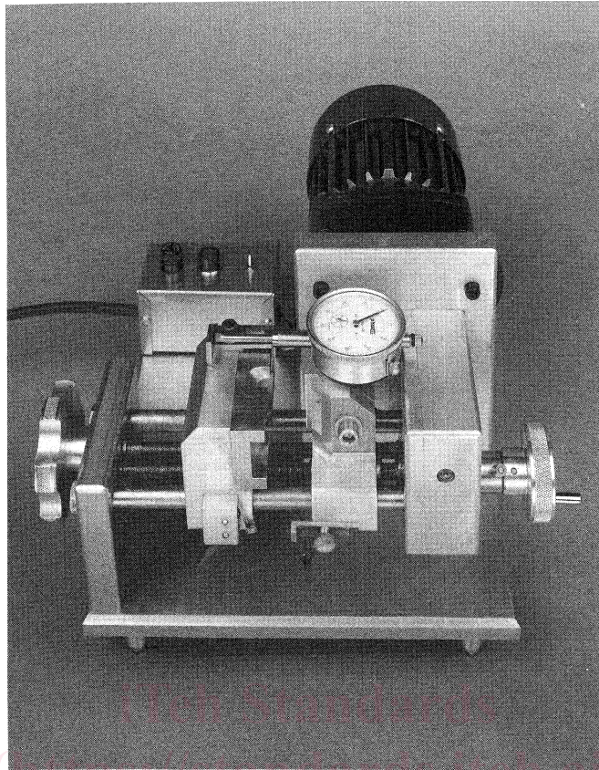
FIG. 2 Notching Machine
