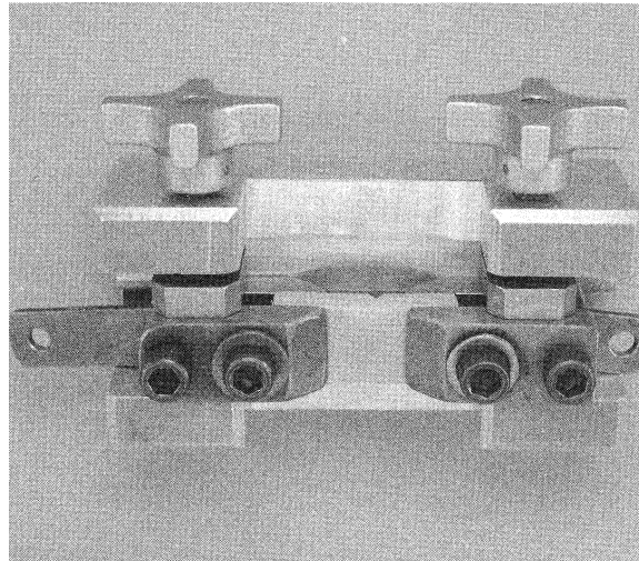
FIG. 1 Alignment Jig
