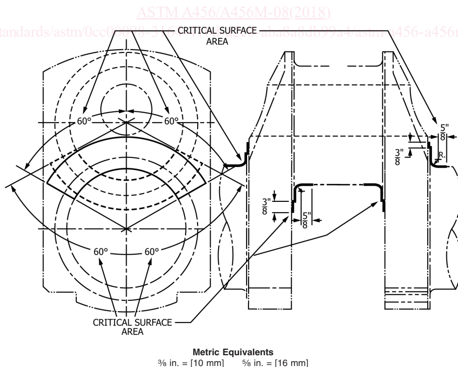
FIG. 1 Critical Surface Areas of Crankpin and Main Bearing Journal
