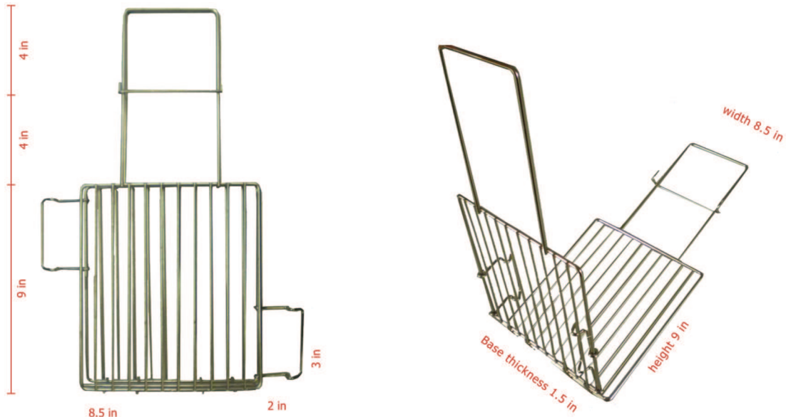
FIG. 1 Food Racks in Rethernalizer Used for Efficiency Tests
