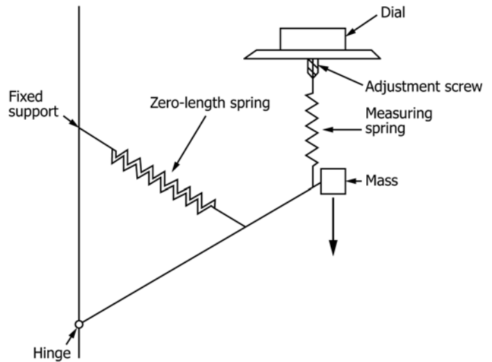
FIG. 1 Gravimeter (from Milsom (4))
