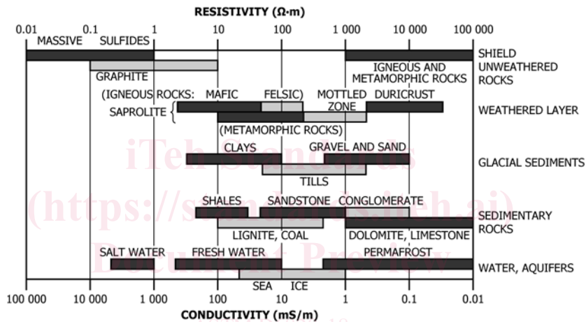
FIG. 6 Typical Ranges of Resistivities and Conductivities of Earth Materials (5)
