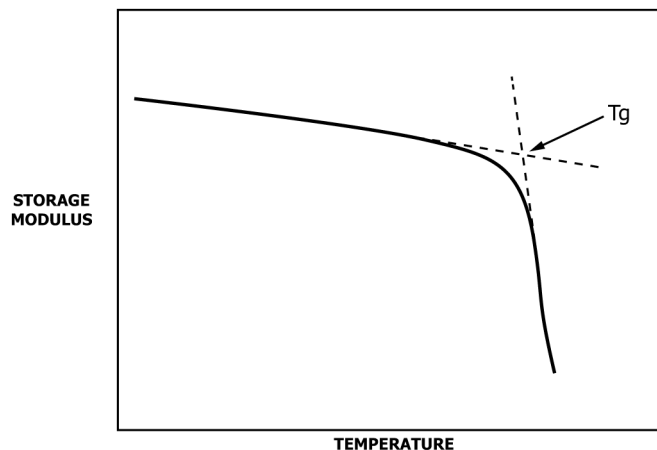
FIG. 1 Storage Modulus
