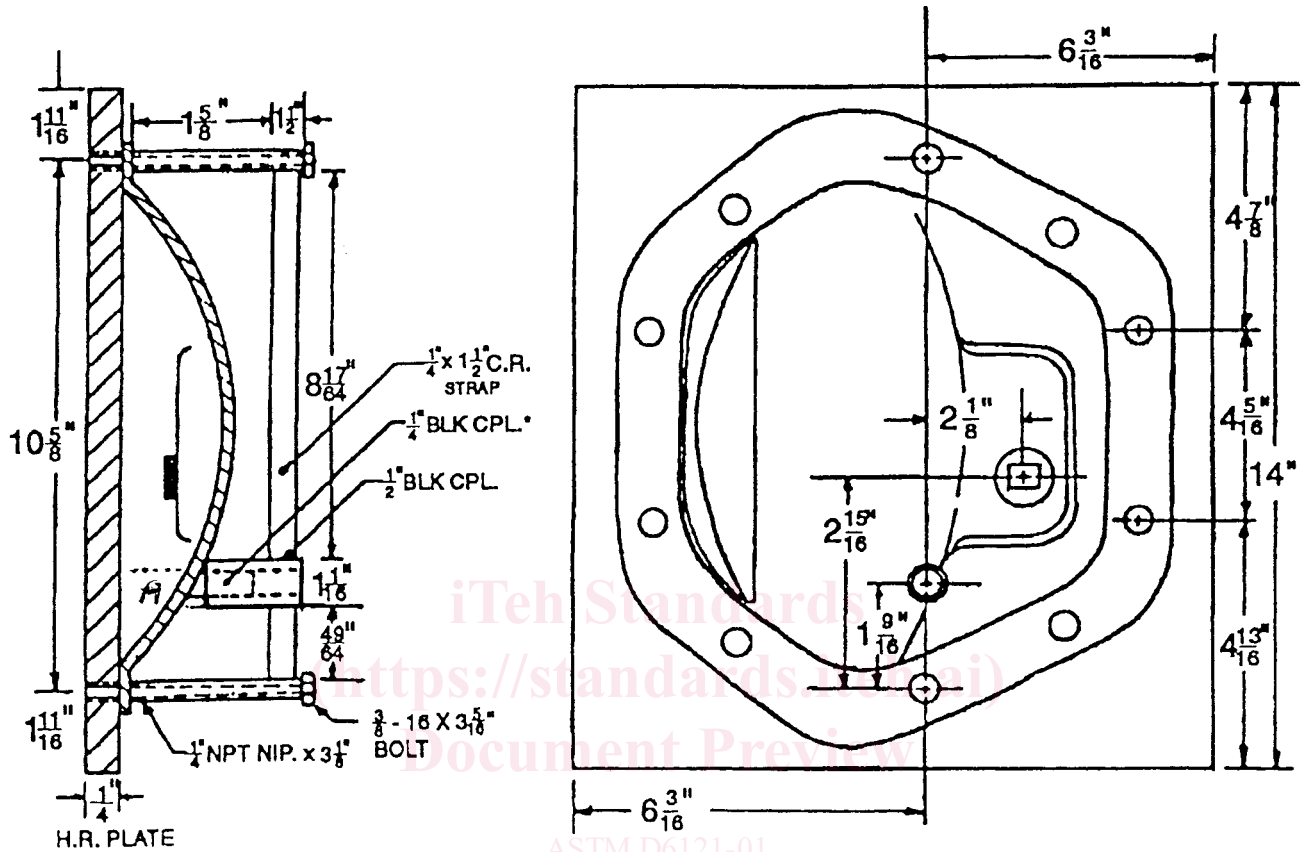
FIG. A4.1 Cover Plate Temperature Sensor Locating Device
