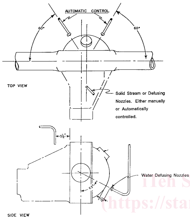
FIG. A5.1 Location of Spray Nozzles on Axle
