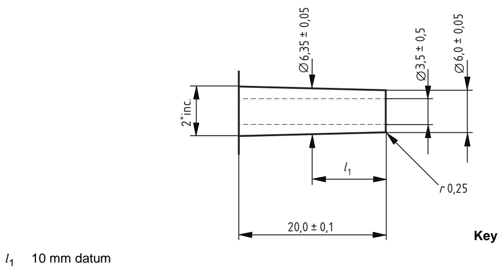
Figure A.1 — Test nipple made in stainless steel : fine-ground finish N6
