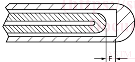
FIG. 2 Ungrounded Measuring Junction, Style U
