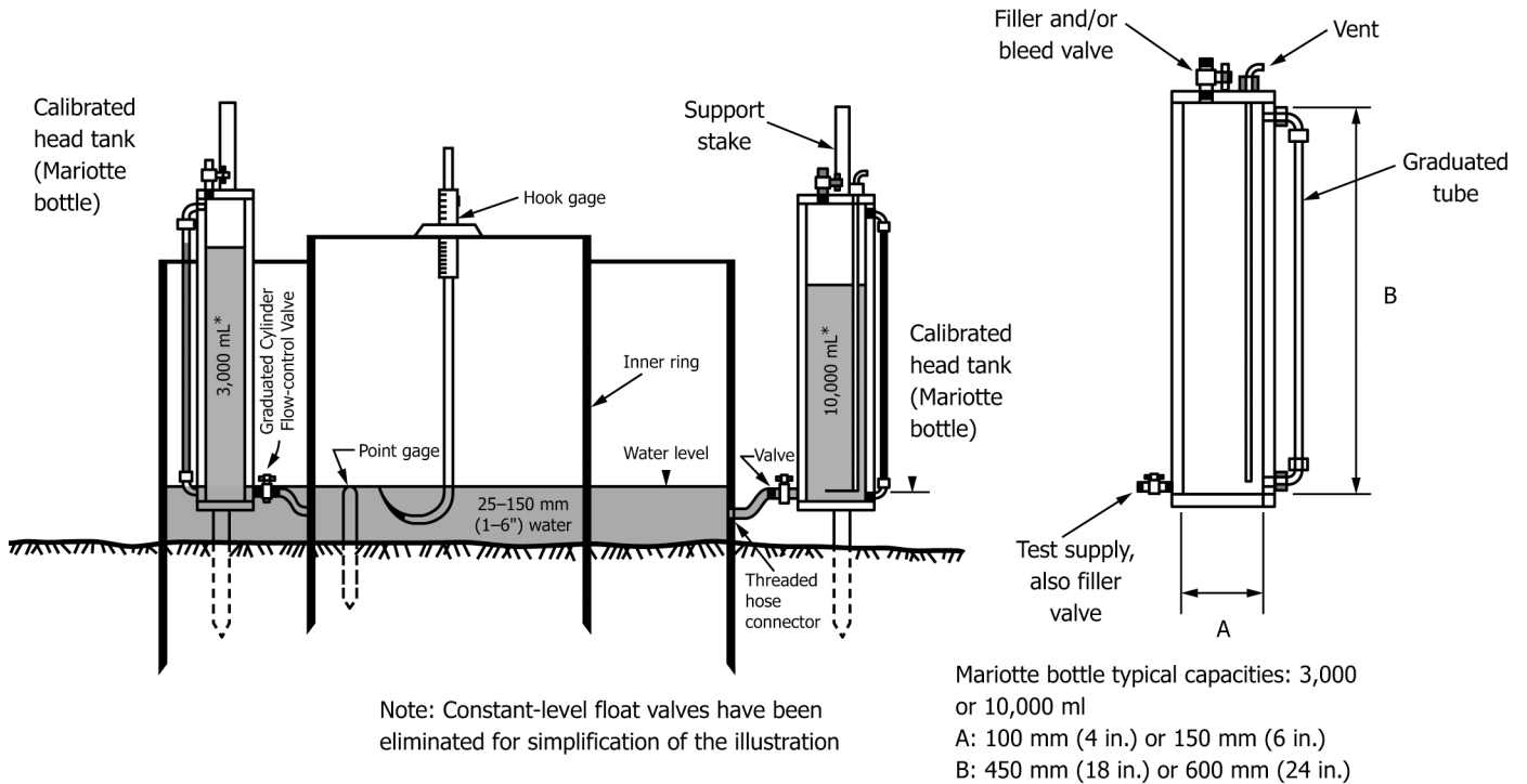
FIG. 2 Ring Installation and Mariotte Tube/Bottle Details
