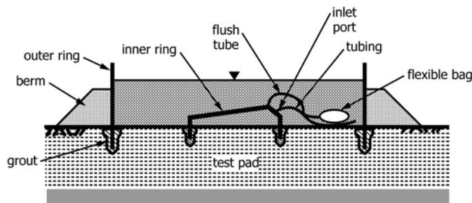
FIG. 1 Schematic Of A Double-Ring Infiltrimeter With A Sealed Inner Ring
