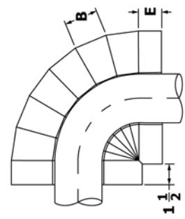
Figure 1.2 Negative Radius Ell
