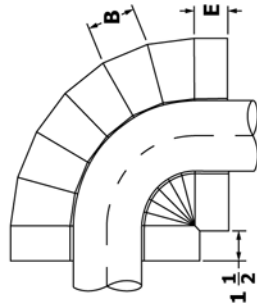
Figure 1.2 Negative Radius Ell
