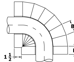
Figure 1.2 Negative Radius Ell
