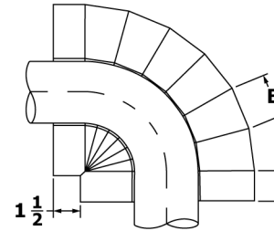
Figure 1.2 Negative Radius Ell
