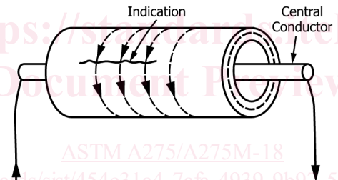
FIG. 4 Circular Magnetization, Current Through a Conductor
