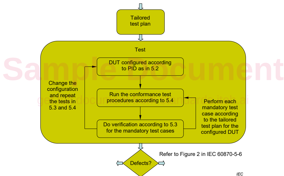
Figure 1 – Test procedure
