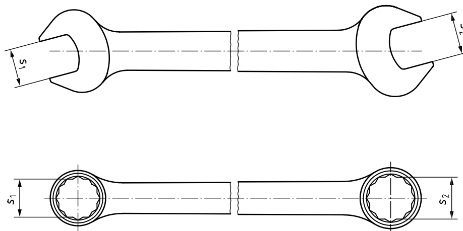
Figure 1 — Double-ended wrenches
