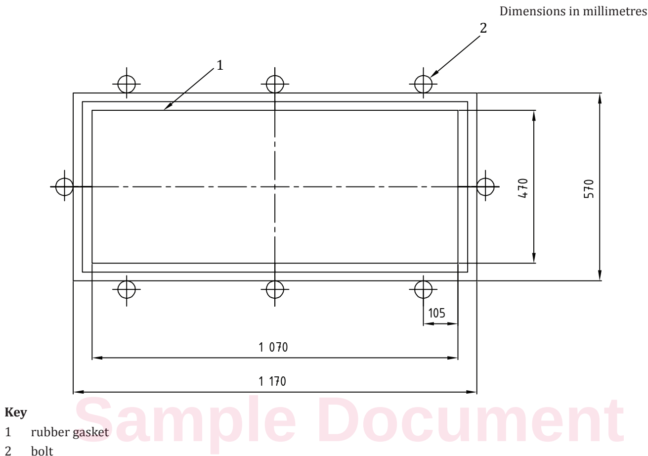
Figure 2 — Support for head-form tests
