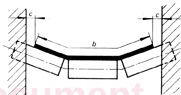
FIGURE 1 — Carrying idlers
