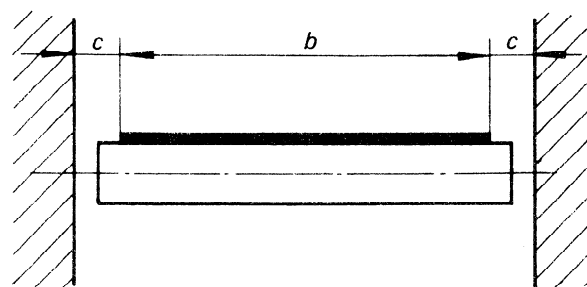
FIGURE 2 — Return idler
