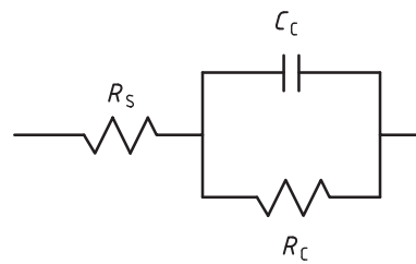
Figure 3 — Randles equivalent circuit
