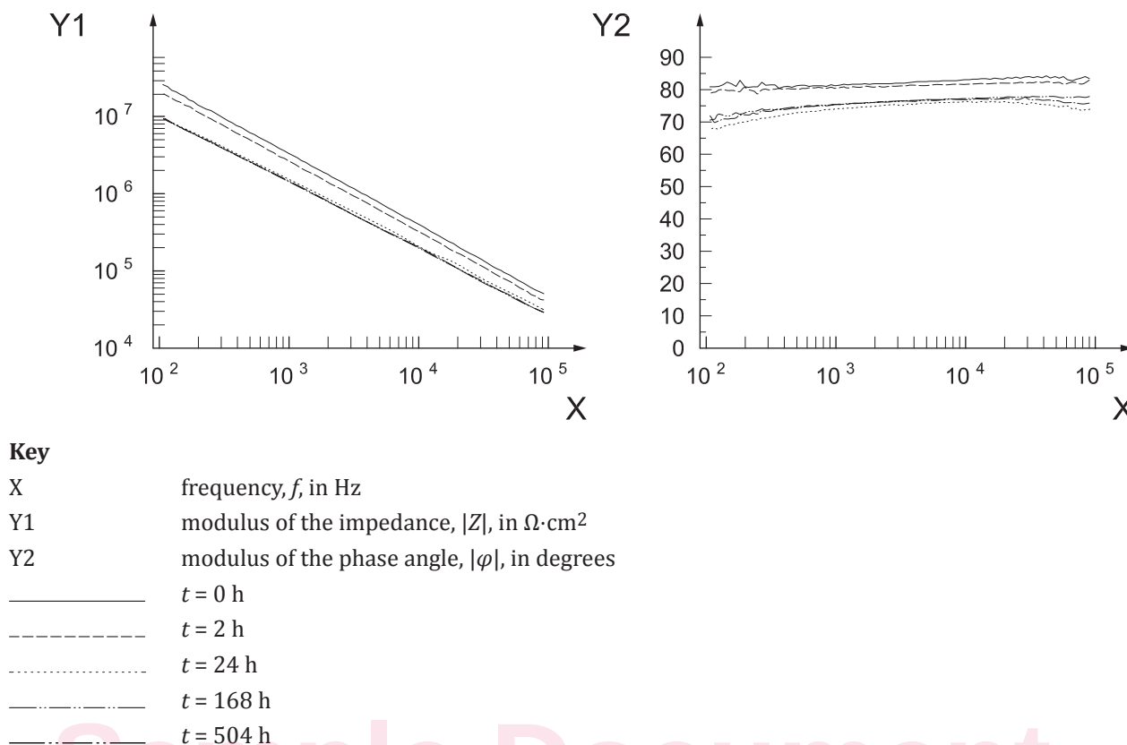
Figure A.2 — Bode plot for a surface-tolerant coating material under immersion conditions
