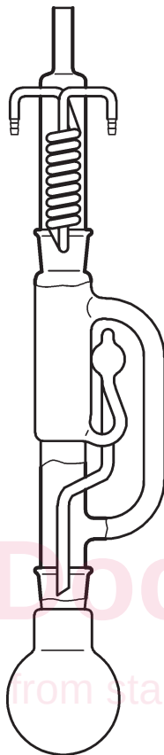
Figure 1 — Extraction apparatus
