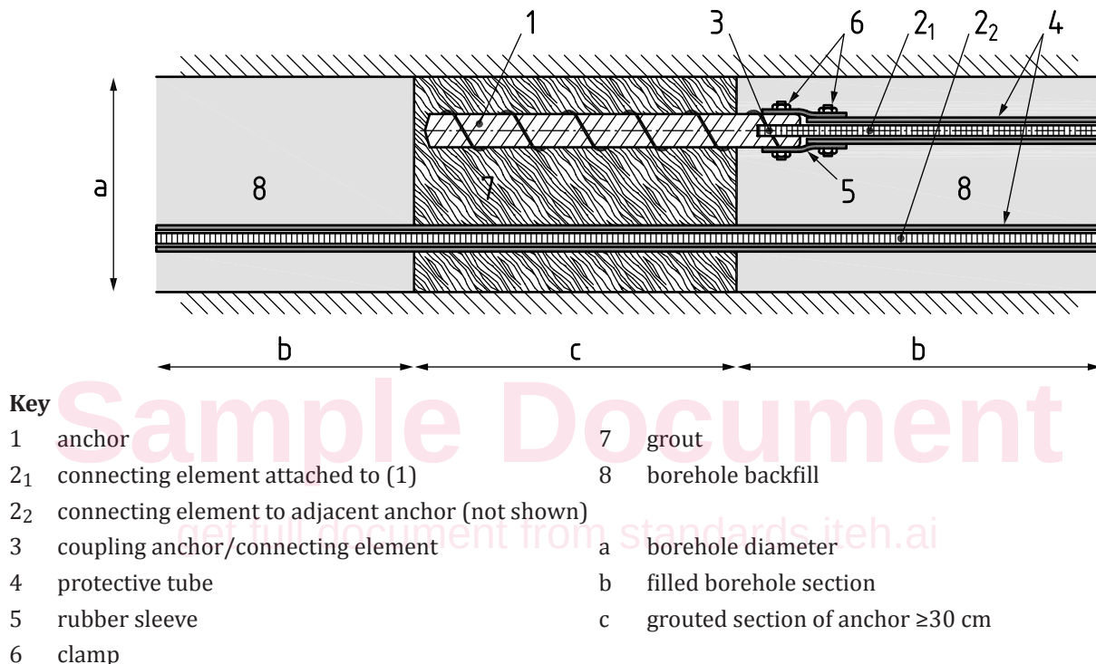
Figure 4 — Example of a cement-grouted anchor of a multiple-point borehole rod extensometer with the connecting element attached to the anchor and a passing connecting element
