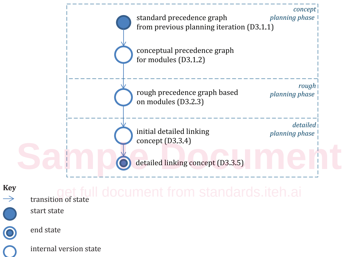
Figure 8 — States of the precedence graph information object
