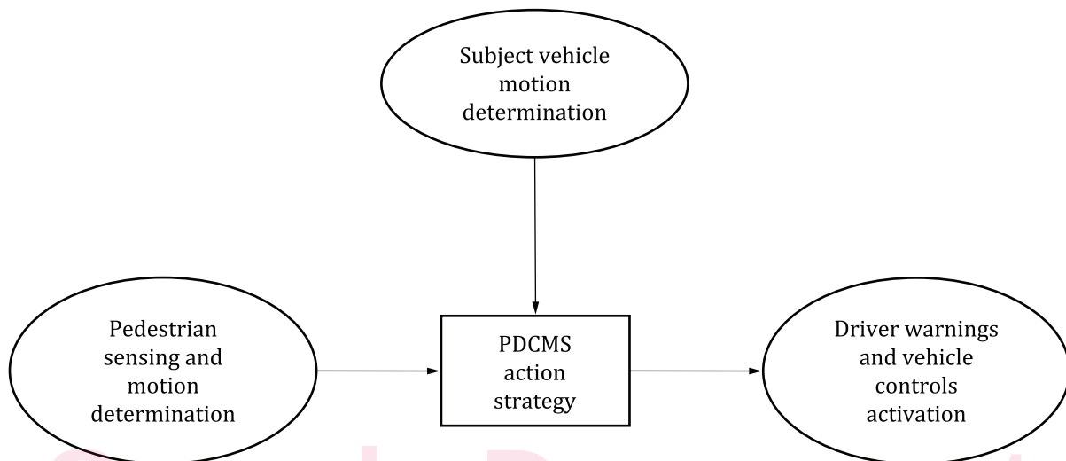
Figure 1 — Functional elements of pedestrian detection and collision mitigation systems (PDCMS)
