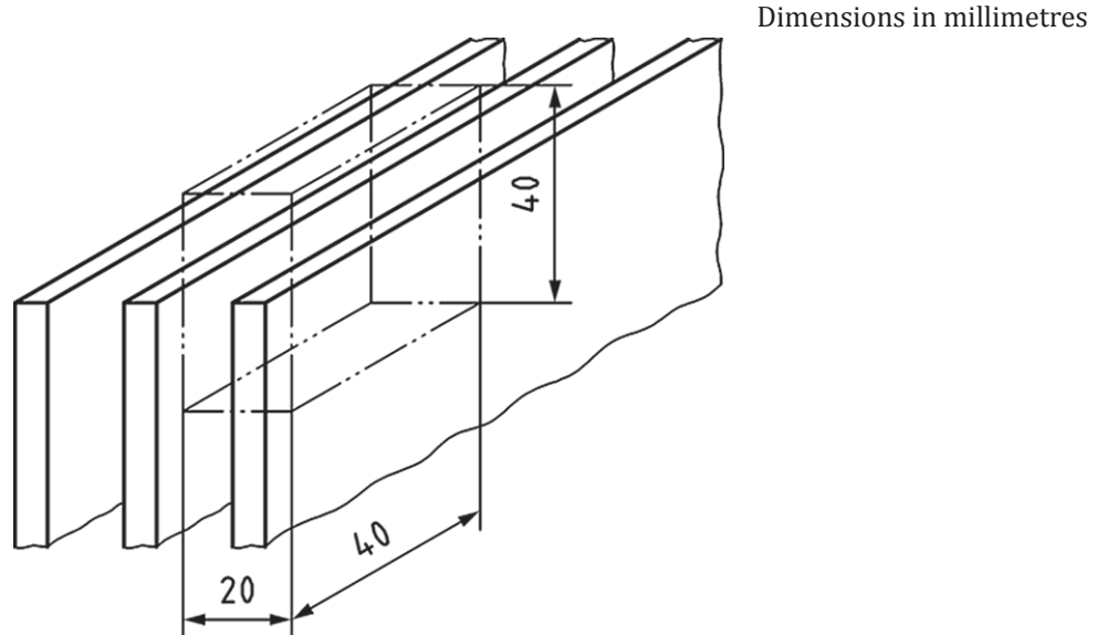
Figure 2 — Example of a vertical glass separator
