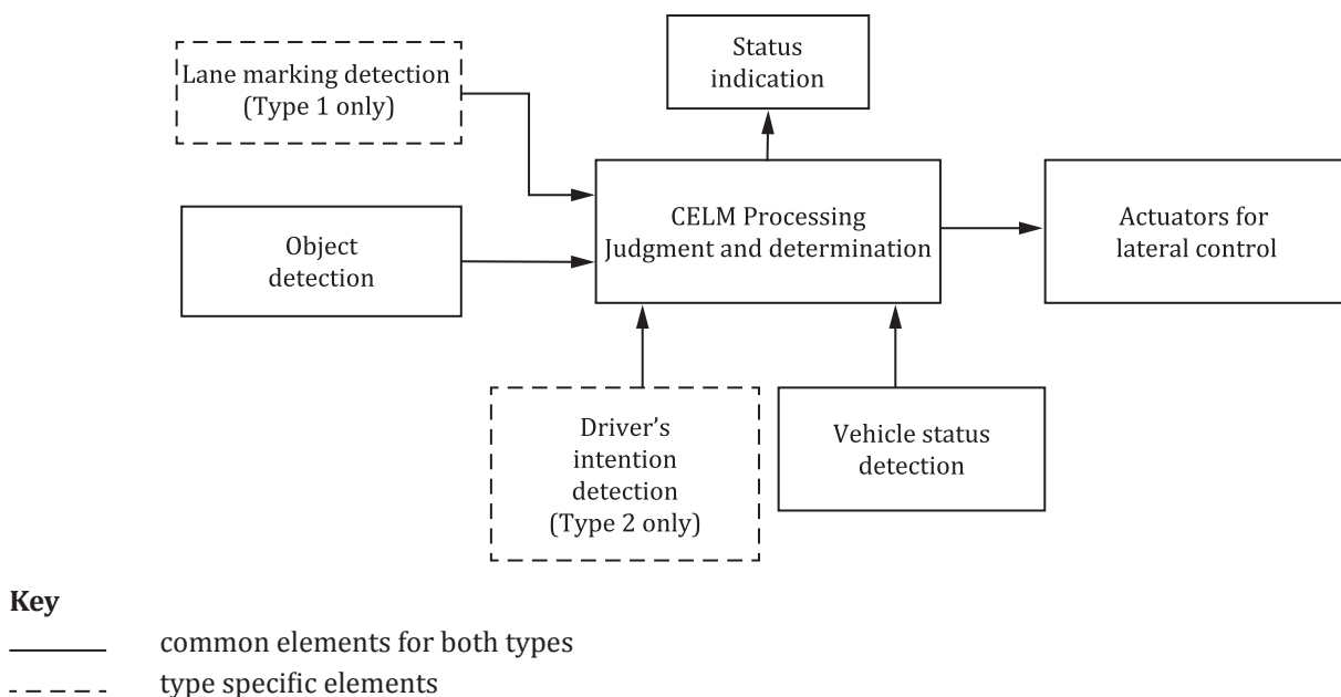
Figure 1 — Functional elements
