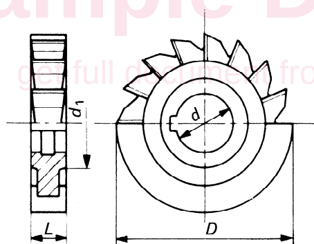
FIGURE 1 — Cutter with straight teeth
