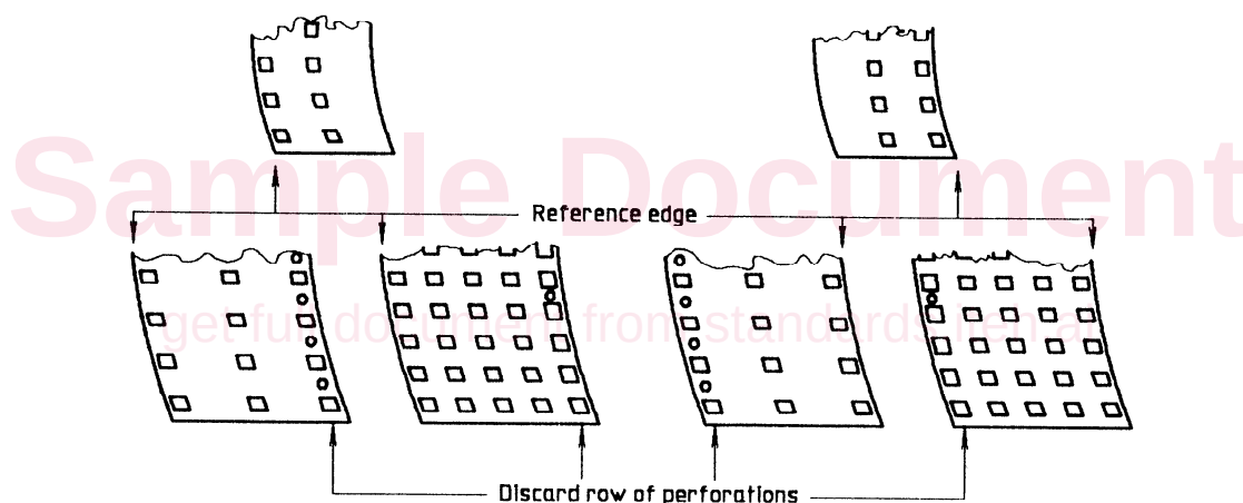
Figure 1 — Reference edge and discarded row designation
