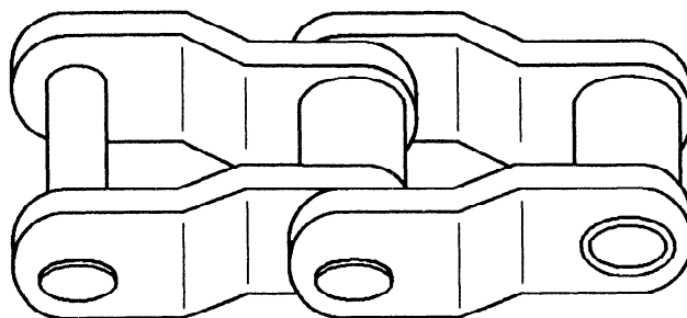
Figure 1 — Cranked-link chain assembly
