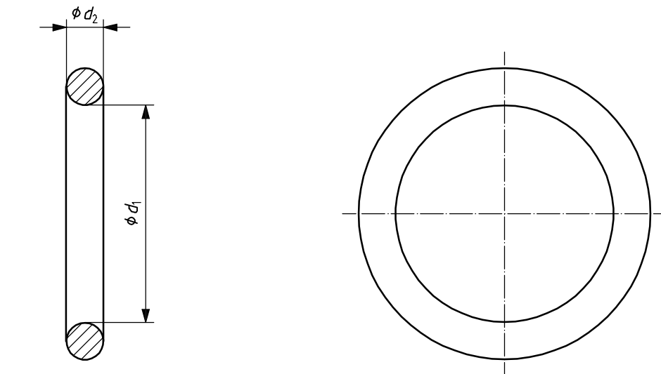
Figure 1 — Typical O-ring configuration
