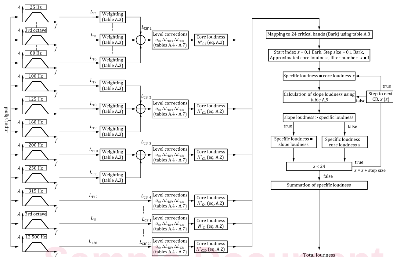
Figure 1 — Block diagram of the calculation method by this document, method for stationary sounds
