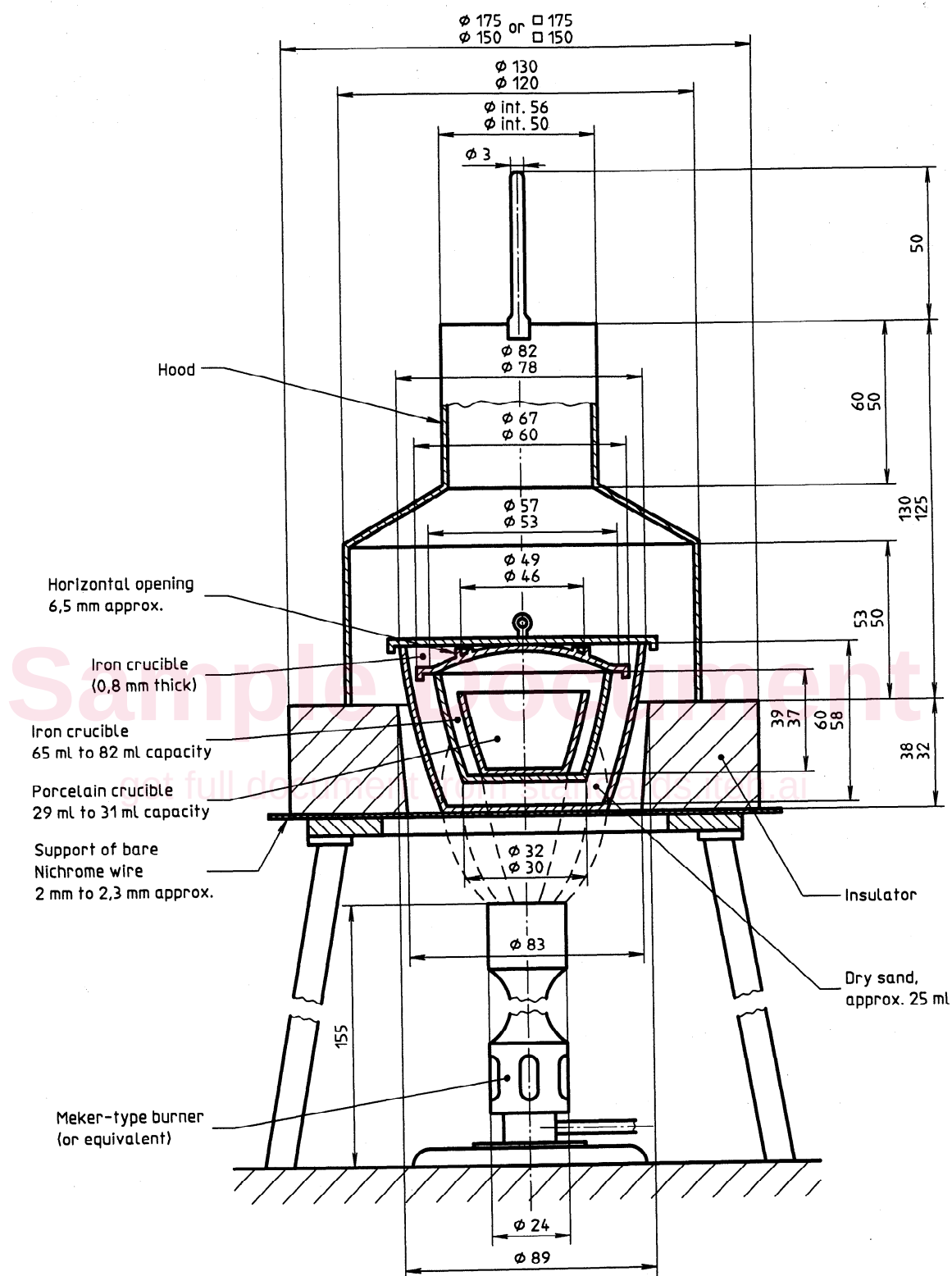
Figure 1 — Apparatus for determining Conradson carbon residue
