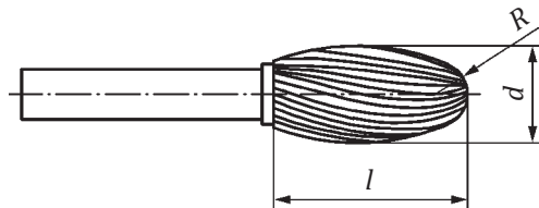
Figure 1 — Hardmetal burr, style E
