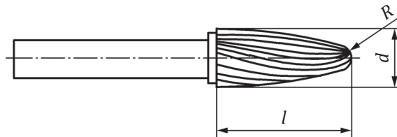
Figure 1 — Hardmetal burr, style F
