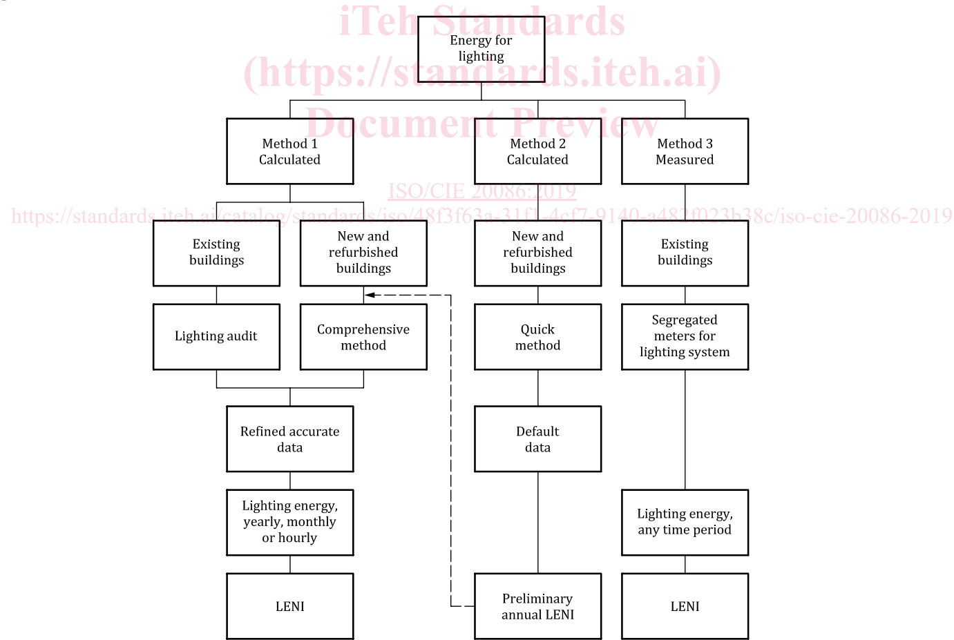
Figure 1 — Flow chart illustrating alternative routes to determine energy use
