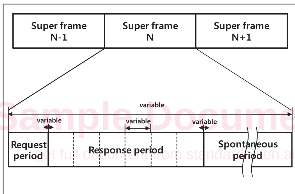
Figure 6 — MFAN superframe structure
