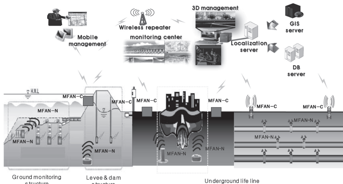
Figure 1 — Underground monitoring system
