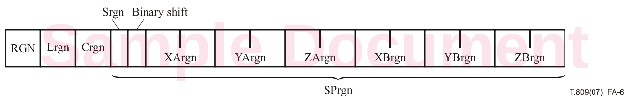
Figure A.6 – Region-of-interest syntax
