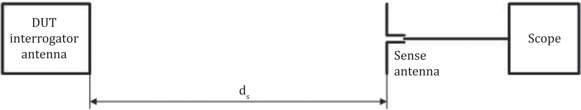
Figure 1 — Interrogator modulation test setup
