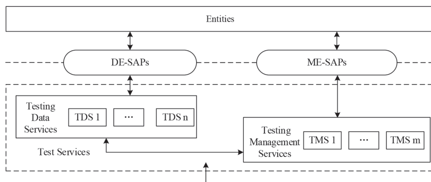
Figure 4 — Overview of test services for sensor networks
