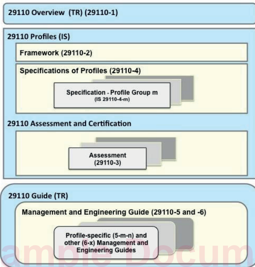
Figure 1 — ISO/IEC 29110 Series
