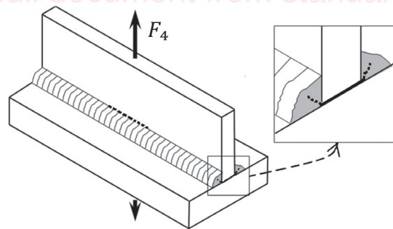
e) Transverse load-carrying fillet weld, root cracking
