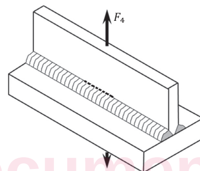
d) Transverse normal load-carrying fillet weld, toe cracking
